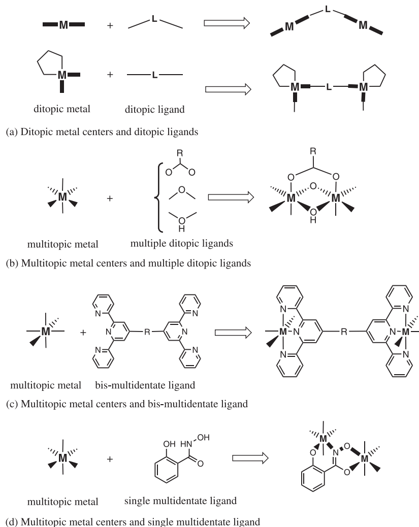
FIGURE 1 Schematic drawings of the types of metal-ligand linkages in metallamacrocycles.
