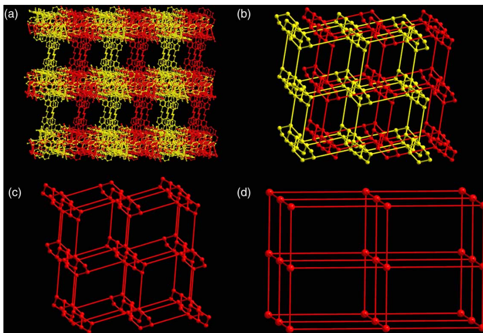
FIGURE 14 Two-fold interpenetrating 3-D network prepared using the hexanuclear manganese metalladiazamacrocycle as a supramolecular hexatopic building block. (a) The packing diagram of the network shows two interpenetrated 3-D nets in red and yellow, where one type of bpea linkers serve as pillars between the interwoven 2-D layers. (b) The schematic drawing of the metal ion connectivity shows the two interpenetrated 3-D nets in red and yellow lines. (c) The diagrammatic representation of the net as a 3-connected 4.12_2 net, where all six metal ions of the hexanuclear macrocycle serve as 3-connectivity vertices. (d) The diagrammatic representation of the net as a well known simplified 6-connected simple cubic net, when the metallamacrocycle in the net described in (c) was further reduced to a simple octahedral node (colour in online version).
