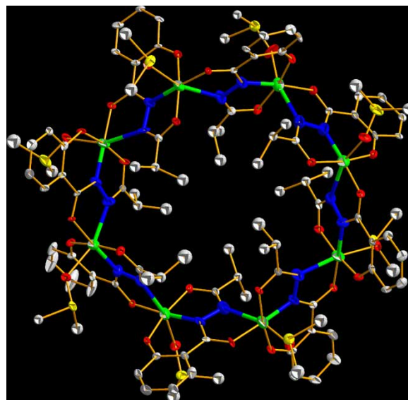
FIGURE 6 ORTEP diagram of an octanuclear metallamacrocycle prepared using a ligand with sterically least demanding two C\beta carbon atoms as terminal N -acyl group. The 24-membered, 8-metal ring system is highlighted with thickened bonds, where the metal ions are presented in green and the bridging nitrogen atoms in blue (see online for colour).
