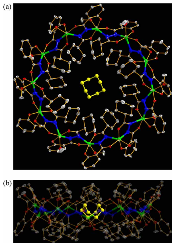
FIGURE 10 ORTEP diagrams of a dodecanuclear metallamacrocycle with \dots(\Lambda\Delta)(\Lambda\Delta)\dots chiral sequence. A cyclooctane guest molecule is induced-fit into the S_{12} symmetry cavity of the macrocycle in a strained S_4 conformation rather than in a relaxed S_8 conformation. (a) Top view. (b) Side view.
