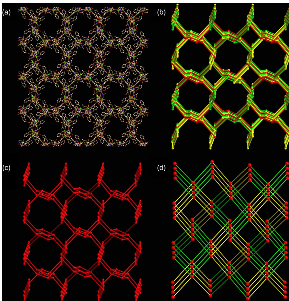
FIGURE 12 Three-fold interpenetrating 3-D network prepared using the hexanuclear manganese metalladiazamacrocycle as a supramolecular tetratopic building block related via 4_1 and 4_3 screw symmetry. (a) The packing diagram of the network shows two different types of channels along the crystallographic c -axis that linked each other to form 3-D cavities. Depending on the length of the N -acyl tails, the size and dimensionality of the cavity could be tuned. (b) The schematic drawing of the metal ion connectivity shows three interpenetrated 3-D nets represented in red, yellow, and green lines. (c) The individual net could be described as 3-connected 4.8.16 net, where only four metal ions of the macrocycle have served as 3-connectivity vertices. (d) When the metallamacrocycle presented as a rectangle was further reduced to a square node, the net described in (c) could be simplified to 4-connected 4^2.8^4 net.
