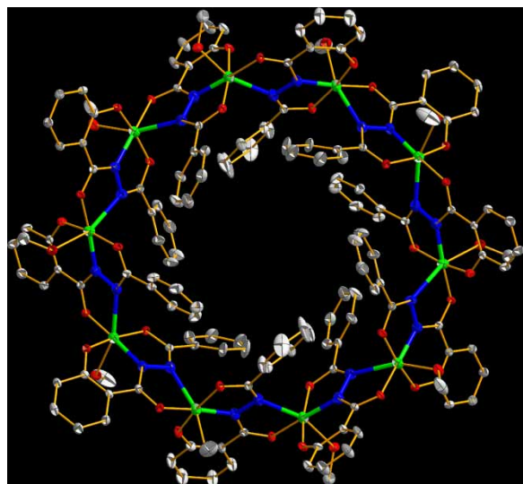
FIGURE 7 ORTEP diagram of a decanuclear metallamacrocycle with phenyl group as the N -terminal group. The 30-membered, 10-metal ring system was highlighted with thickened bonds, where the metal ions were presented in green and bridging nitrogen atoms in blue (see online for colour).
