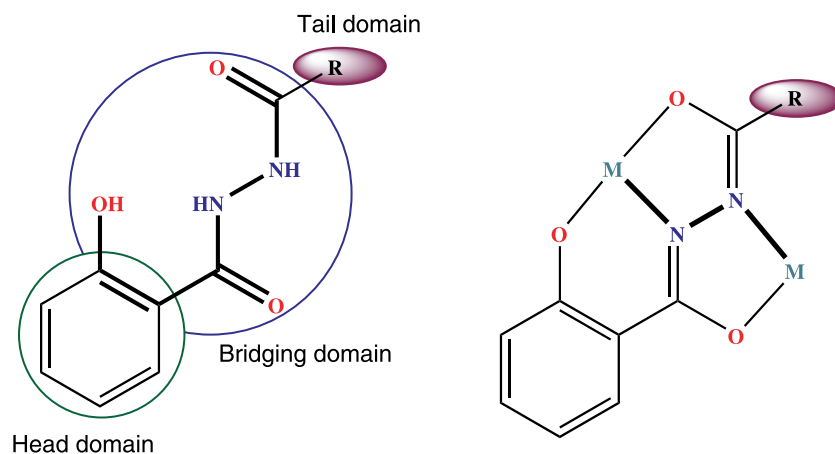
FIGURE 2 Schematic diagrams representing three domains of the ligand, N -acylsalicylhydrazide and its bridging mode.
