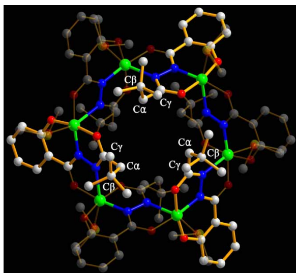
FIGURE 5 Ball and stick representation of a hexanuclear metallamacrocycle showing the close contact interaction between C_3 symmetric positioned N -acyl tail groups (see online for colour).
