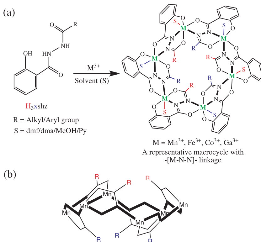
FIGURE 3 (a) The reaction scheme for the preparation of metalladiazamacrocycles. (b) Schematic side view represents the steric interaction between the N -acyl tail domains of the ligands.
