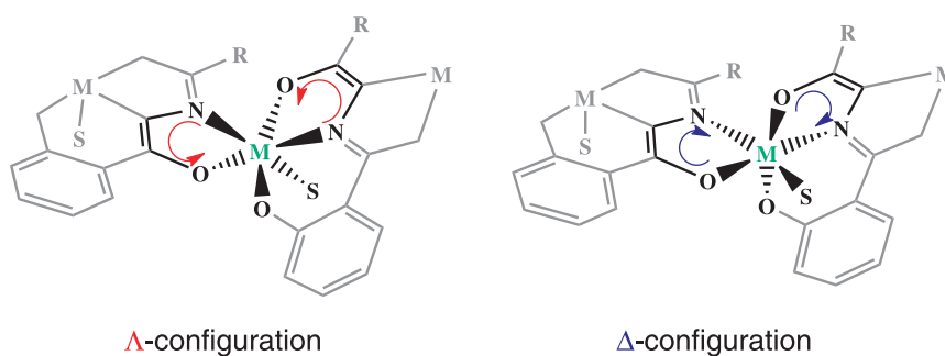
FIGURE 4 Schematic representation of the chiral configuration around metal center.
