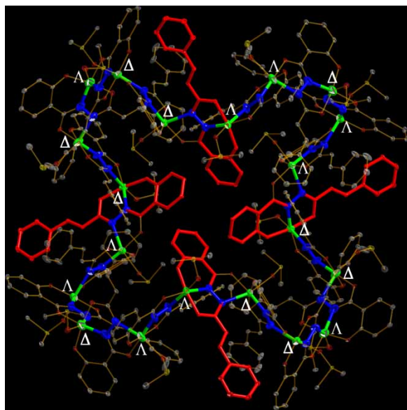
FIGURE 9 ORTEP diagram of an icosanuclear metallamacrocycle with \dots(\Lambda\Lambda\Delta\Lambda\Delta\Delta\Lambda\Delta\Delta)\dots chiral sequence. The 60-membered, 20-metal ring system was highlighted with thickened bonds, where the metals were presented in green and bridging nitrogen atoms in blue. Four out of twenty ligands are in rather unusual 'inverted' conformation, where the phenyl 'head domain' of the ligand is located around the inner core of the macrocycle to reduce the steric repulsion (see online for colour).
