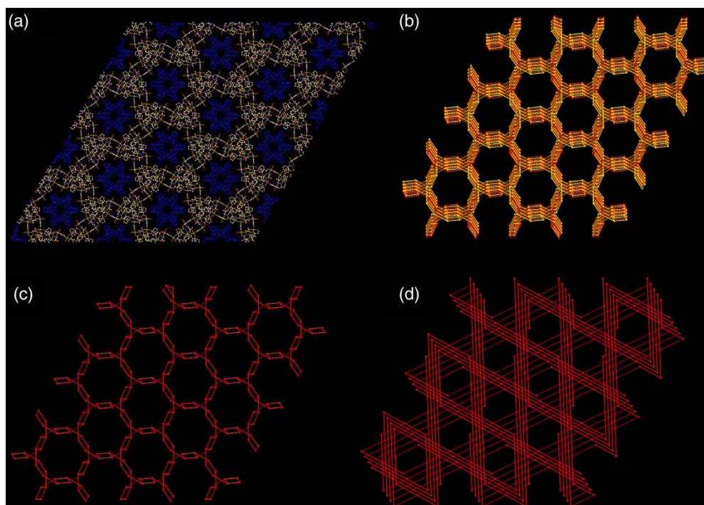
FIGURE 13 Two-fold interpenetrating 3-D network prepared using the hexanuclear manganese metalladiazamacrocycle as a supramolecular tetrapodal building block related via 3 1 and 3 2 screw symmetry. (a) The packing diagram of the network shows 1-D channels along the crystallographic c -axis, where the metallamacrocycles (in blue) unconnected to the framework were stacked to fill the channel cavity. (b) The schematic drawing of the metal ion connectivity shows the two interpenetrating 3-D nets in red and yellow lines. (c) The representation showing the individual net as a 3-connected 4.12 2 net, where again only four metal ions of the hexanuclear macrocycle serve as 3-connectivity vertices. (d) Diagrammatic representation of the simplified 4-connected 6 4 .8 2 net, when the metallamacrocycle presented as a rectangle in (c) was further reduced to a square node.
