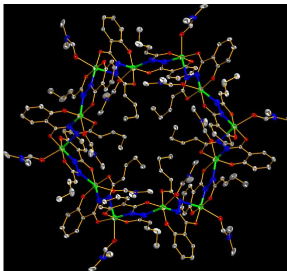
FIGURE 8 ORTEP diagram of a puckered dodecanuclear metallamacrocycle with \dots(\Lambda\Lambda\Delta\Delta)(\Lambda\Lambda\Delta\Delta)\dots chiral sequence. The 36-membered, 12-metal ring system was highlighted with thickened bonds, where the metals were presented in green and bridging nitrogen atoms in blue (see online for colour).
