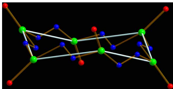
FIGURE 11 The core of a hexanuclear metalladiazamacrocycle emphasizing the hexatopic nature as a supramolecular building block, where the metals were presented in green, the bridging nitrogens in blue, and the solvents ligated to the metal ions in red. The ring metal ions in the cyclohexane-like chair conformation with the replaceable solvents can serve as the potential triangular nodes in the metal-organic frameworks.
